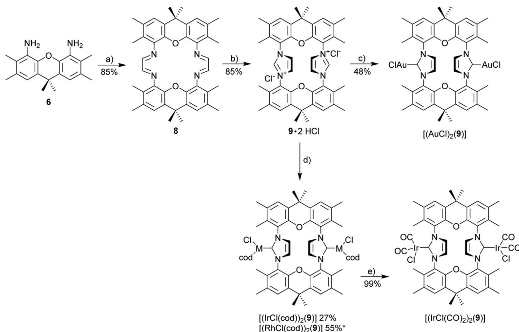
Scheme 3 Synthesis of azolium salt 9 ·2HCl and derived metal complexes. Reagents and conditions: (a) glyoxal, p\text{TsOH} , n\text{BuOH} , 50^\circ\text{C} ; (b) paraformaldehyde, \text{Me}_3\text{SiCl} , \text{EtOAc} , 70^\circ\text{C} , 24 h; (c) \text{Ag}_2\text{O} , \text{MeOH} , rt, 24 h then [\text{AuCl}(\text{SMe}_2)] , 50^\circ\text{C} , 2 h; (d) [\text{MCl}(\text{cod})_2] ( \text{M} = \text{Ir}, \text{Rh} ), sodium amylate, THF, -78^\circ\text{C} ; (e) \text{CO} , 0^\circ\text{C} , \text{CH}_2\text{Cl}_2 30 min; (* yield of crude complex).
