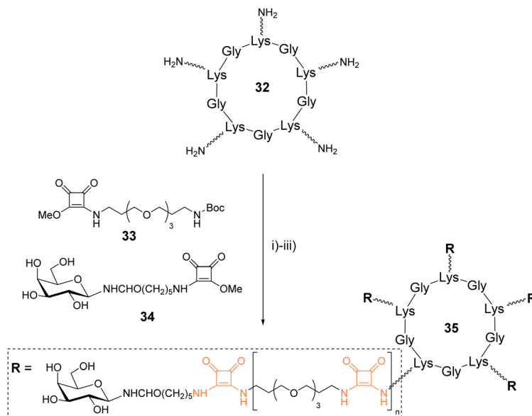
Scheme 5 Synthesis of glycoclusters using squaramide coupling. Reagents and conditions: (i) 33 , \text{NaHCO}_3 , \text{H}_2\text{O}/\text{CH}_3\text{OH} ; (ii) 34 , \text{NaHCO}_3 , \text{H}_2\text{O}/\text{CH}_3\text{OH} , approx. 70%.
