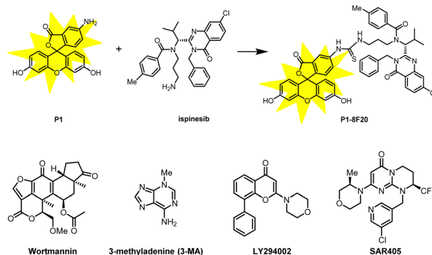
Fig. 16 The FITC-ATTEC fluorescent probe and typically used lysosome and autophagosome inhibitors.
