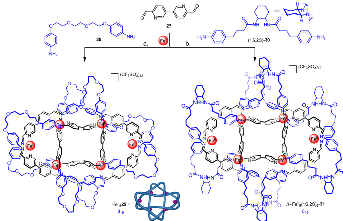
Fig. 10 (a) Synthesis of racemic 8_{19} knot \text{Fe}_6^{\text{II}}\text{29} from dianiline 28 . (b) Synthesis of 8_{19} knot \Lambda\text{-Fe}_6^{\text{II}}(1\text{S},2\text{S})_6\text{-31} from enantiopure dianiline (1\text{S},2\text{S})\text{-30} . 60
