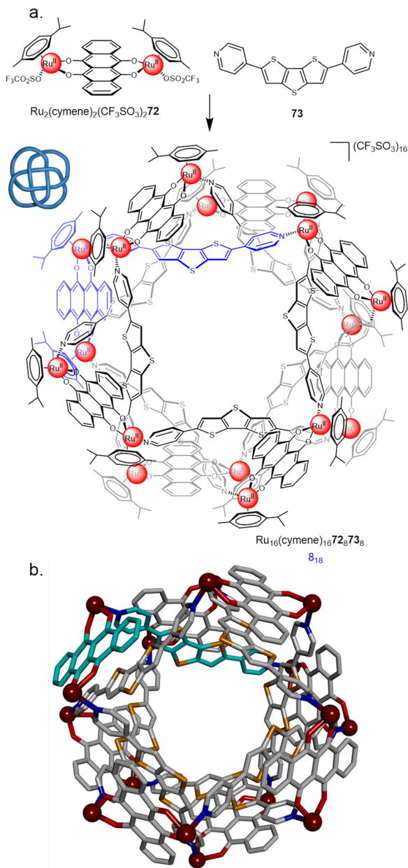
Fig. 25 (a) Synthesis of 8_{18} metalla-knot Ru_{16}(p\text{-cymene})_{16}72_873_8 . (b) X-ray crystal structure of the 8_{18} metalla-knot with p -cymene ligands omitted for clarity. 100
