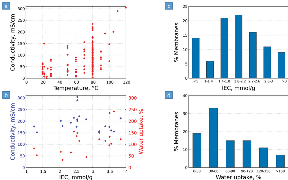
Fig. 10 (a) AEM hydroxide conductivity vs. temperature, and (b) hydroxide conductivity and water uptake of selected AEMs (with conductivities \geq 150 mS cm ^{-1} ). (c) Fraction of AEMs at different levels of (c) IEC range and (d) water uptake range. Water uptake values are given in different temperatures. Represented data and the underlying sources are given in Table S1 (ESI ^{\dagger} ).
