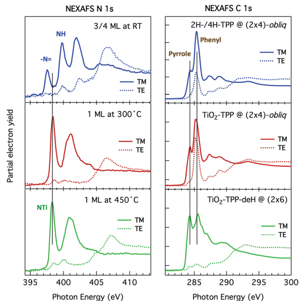
Fig. 17 NEXAFS spectra measured in partial electron yield at the N and C K-edges, left and right panels, respectively, at RT, 300 °C and 450°, corresponding to different molecular species and symmetry phases; spectra measured in TM and TE polarization are represented as full and dotted lines, respectively. The surface was azimuthally oriented to keep the scattering plane along the [001] direction. In this geometry, the TE spectra are measured with the electric field transverse to the rows, where the molecules display a slightly larger intensity of \pi -symmetry resonances than along the rows, hence yielding the maximum tilt angle/molecular distortion in any chemical state. Adapted from ref. 49 with permission from the Royal Society of Chemistry, Copyright 2017.
