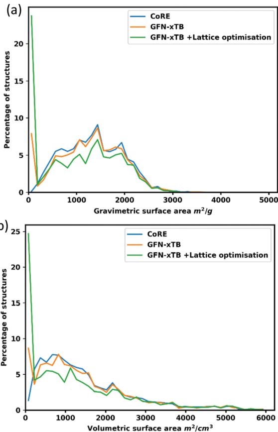
Fig. 5 (a) Gravimetric and (b) volumetric accessible surface areas of CoRE structures, as provided (blue) and after optimization using GFN-xTB in AMS with fixed lattice parameters and relaxed lattice parameters (orange and green respectively).
