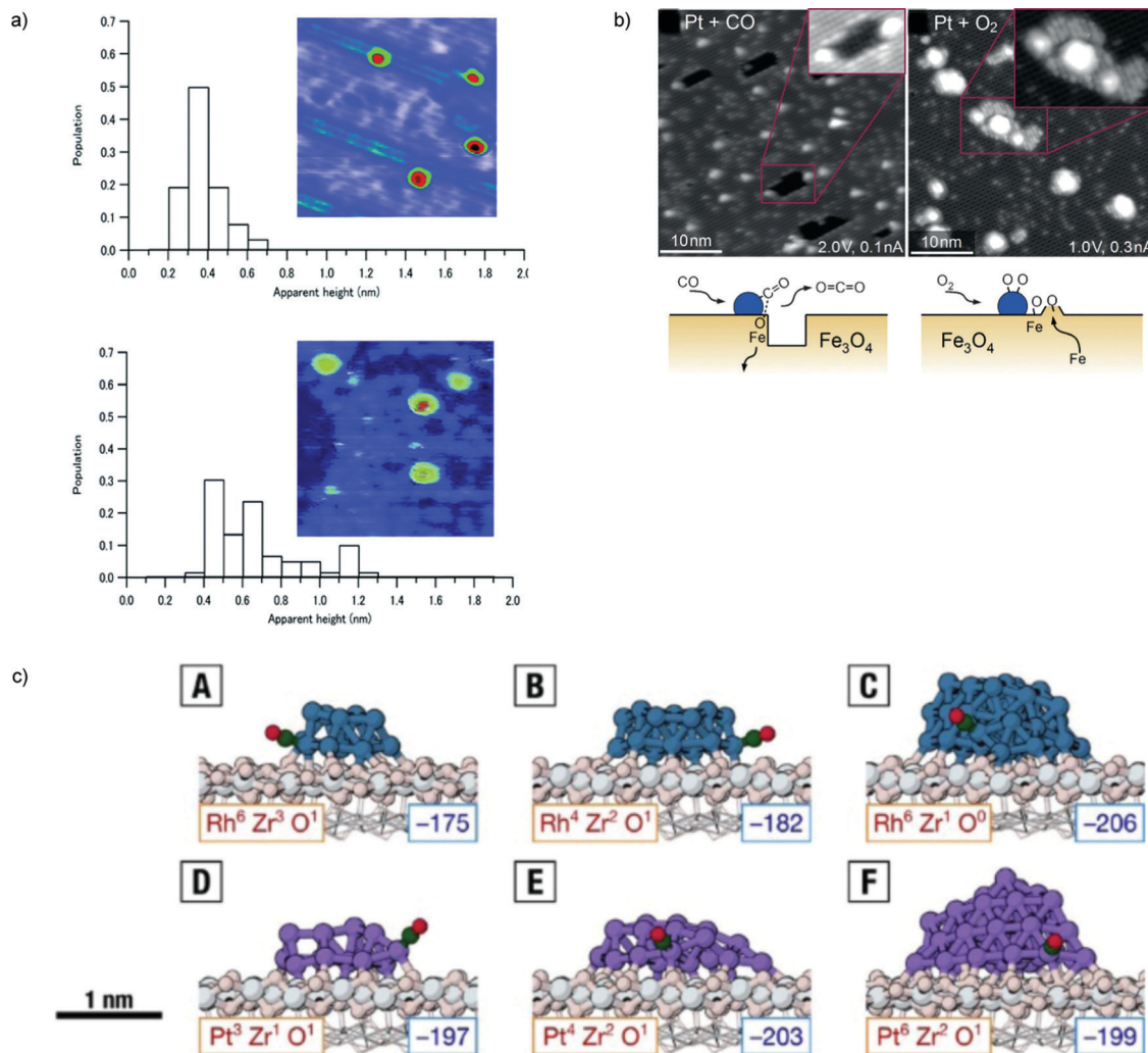
Fig. 7 (a) Histograms of apparent height and STM topographic images ( 24 \times 24 \text{ nm}^2 , 3.5 \text{ V}_s , 100 \text{ pA} ) of as-deposited size-selected Pt 10 clusters under vacuum at 27^\circ\text{C} (upper part) and after CO and O 2 exposure at 27^\circ\text{C} (lower part). (b) STM images acquired following exposure of the Pt/Fe 3 O 4 (001) model catalyst to 1 \times 10^{-7} mbar of CO (left), or O 2 (right) at 550 K. Following exposure to CO (60 min), approximately 50% of the Pt clusters sit at the edge of or inside monolayer holes in the Fe 3 O 4 (001) terrace. The rows (rotated by 90^\circ ) of the next Fe oct -O layer can be seen inside the holes (inset). The illustration shows how CO extracts O lattice atoms from the cluster perimeter and how CO 2 desorbs from the surface. Undercoordinated Fe atoms diffuse into the Fe 3 O 4 bulk. Following exposure to O 2 (20 min), all Pt clusters reside on top of islands with a step height of 2 \text{ \AA} . On the larger islands, the rows (rotated by 90^\circ ) of the next Fe 3 O 4 (001) layer are clearly visible. The islands result from the spillover of oxygen atoms onto the Fe 3 O 4 support, which react with Fe that diffuses out from the bulk. (c) Most favorable adsorption of a CO molecule onto the perimeter sites of (A) Rh 13 /ZrO 2 , (B) Rh 19 /ZrO 2 , (C) Rh 43 /ZrO 2 , (D) Pt 13 /ZrO 2 , (E) Pt 19 /ZrO 2 , and (F) Pt 43 /ZrO 2 . The corresponding adsorption energies (in \text{kJ mol}^{-1} ) are given in the bottom right corners of the panels. The coordination of the corresponding perimeter sites in the absence of CO is given in the bottom left corner of the panels. Color scheme: Rh in teal, Pt in purple, Zr in light gray, oxide O in pink, and CO in green and red. The fixed layers of the supporting oxide are shown in wireframe. (a) is adapted from ref. 142 with permission from the Royal Society of Chemistry, (b) is adapted with permission from ref. 102, Copyright 2015 Wiley-VCH Verlag GmbH & Co. KGaA, Weinheim, (c) is adapted with permission from ref. 160.
