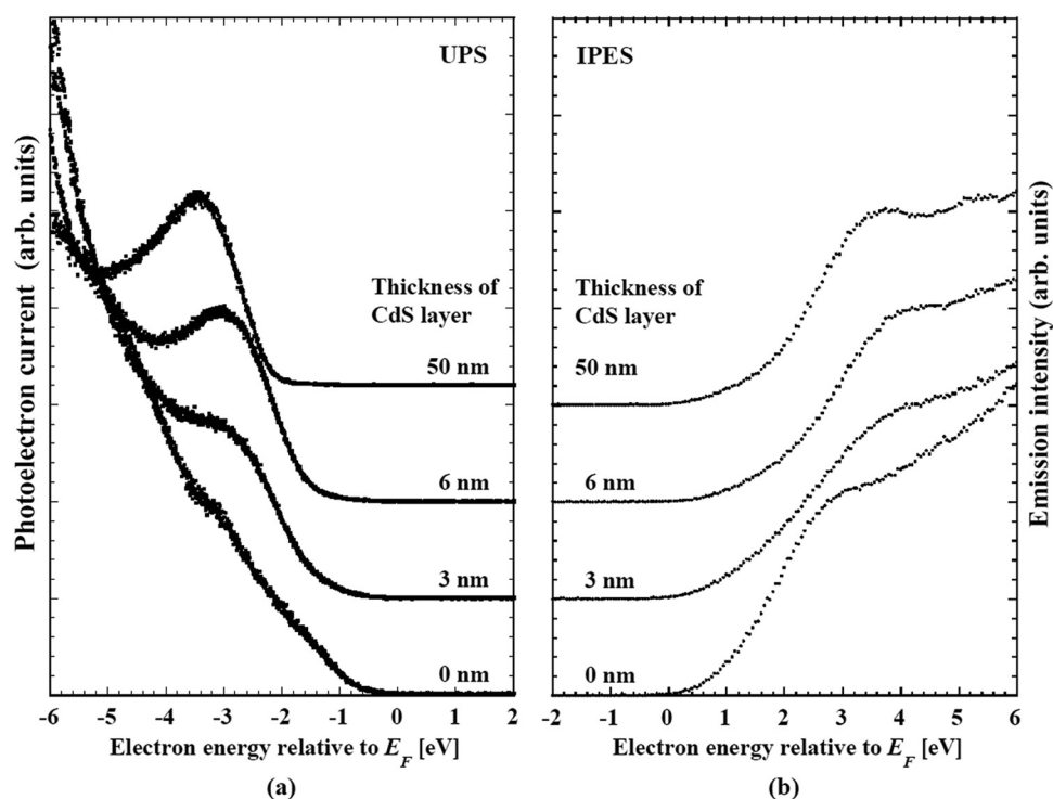
Fig. 20 (a) Changes in the ultraviolet photoemission (UPS) spectra and (b) inverse photoemission (IPES) of CdS-buffer/CIGSSe-absorber structures in conjunction with the thickness of the CdS layer. In both figures, the bottom spectrum indexed with "0 nm" shows nature of the front-surface of the CIGSSe layer.
