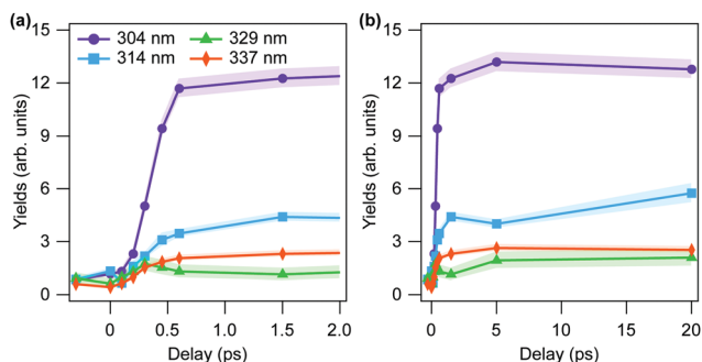
Fig. 2 Experimental results of yields of dissociating molecules in (D + , D + , CO + ) channel at each wavelength as a function of pump-probe time delay (a) between -0.3 ps to 2 ps and (b) up to 20 ps. Hatched areas denote the statistical errors.
