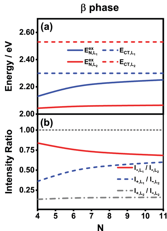
Fig. 7 Analytical results of (a) energies of the FE and CT states and (b) different intensity ratios with respect to the aggregation length for the \beta -phase aggregates. The thin black dashed line in (b) is used to mark the position 1.00 for comparison purposes. The indexes L_1 and L_2 are used to distinguish the two categories of the states in the effective four-state model.
