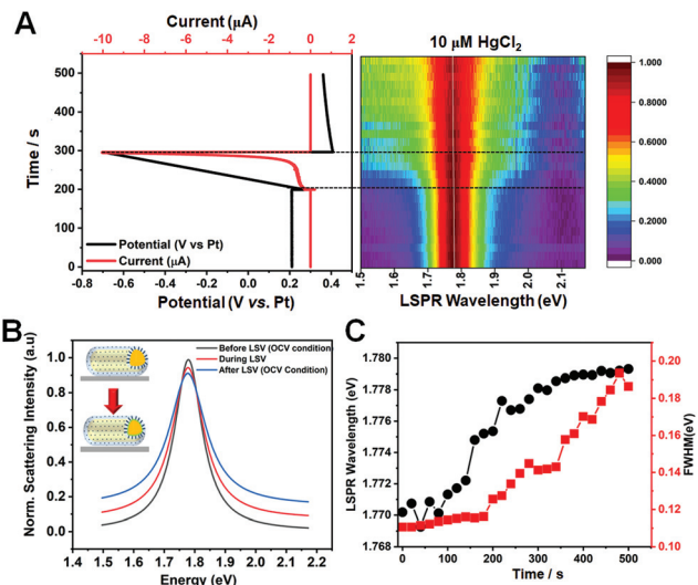
Fig. 5 (A) Potential vs. time and current vs. time curves correlated with a 2D plot of 500 scattering spectra recorded in situ at a single AuNR@mSiO 2 in 0.1 M KCl and 10 μM HgCl 2 . The applied potential was initially held at 0.2 V ( vs. Pt) and then 0.3 V ( vs. Pt), followed by the application of linear cathodic potential sweeps from 0.3 to −0.7 V ( vs. Pt) and, finally, open-cell voltage conditions. (B) Scattering spectra of a AuNR@mSiO 2 before (black curve), during (red curve), and after (blue curve) LSV. (C) LSPR wavelength and FWHM shifts as functions of time during the application of potential energy.
