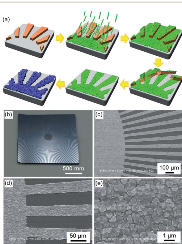
Fig. 3 Fabrication of oriented Cu 3 (BTC) 2 MOF patterns. (a) Schematics showing the fabrication process. The photoresist patterns (orange blocks) were fabricated on the Si wafer using a standard UV lithography method. The Cu(OH) 2 (green rectangles) oriented thin film was deposited onto the Si wafer with the photoresist patterns. The photoresist patterns on which Cu(OH) 2 was deposited were removed by ultrasonic treatment in acetone. The resulting oriented Cu(OH) 2 patterns were converted into oriented Cu 3 (BTC) 2 (blue cuboctahedron-shaped crystal) patterns. (b–e) Photo and SEM images of the oriented Cu 3 (BTC) 2 patterns. In this film, the longitudinal direction ( a -axis) of the underlying Cu(OH) 2 nanobelts is aligned horizontal to the images.
