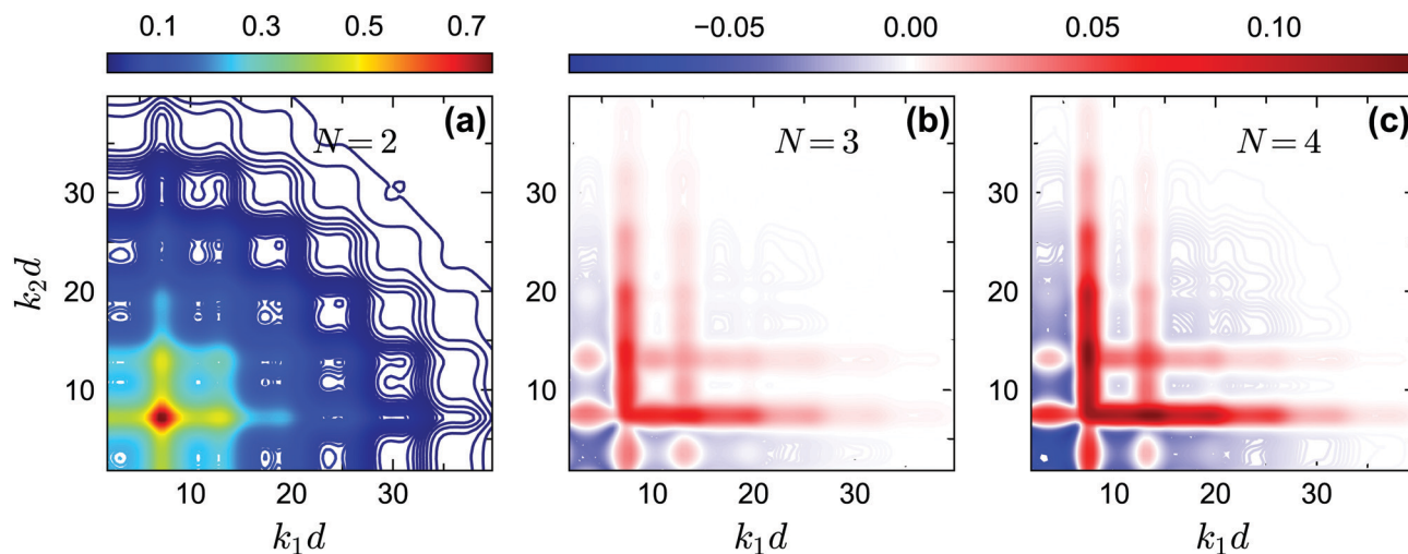
Fig. 6 (a) Non-ergodicity parameters f_2^z(k_1, k_2) as a function of wavenumbers k_1 and k_2 at the critical packing fraction for closure level N=2 (i.e., standard MCT) at \theta = 0.2 and \delta = 0.03 . The patterns of f_2^z(k_1, k_2) from N=3 and N=4 are similar. (b) The difference of the non-ergodicity parameters f_2^z(k_1, k_2) of closure level N=3 with respect to N=2 . (c) The difference of the non-ergodicity parameters f_2^z(k_1, k_2) of closure level N=4 with respect to N=2 . The packing fractions are the same as in Fig. 5.
