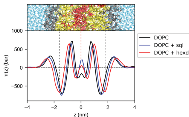
Fig. 4 Lateral pressure profiles for DOPC bilayers with and without hydrophobic solvents. Pure DOPC (black), DOPC/sqI (blue) and DOPC/hexd (red).
