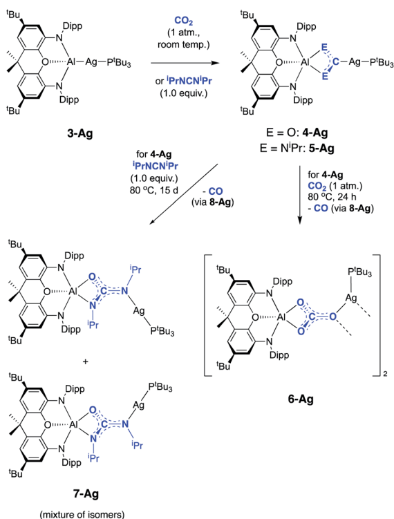
Scheme 3 Reactions of silver–aluminium compound 3-Ag with \text{CO}_2 and ^1\text{PrNCN}^1\text{Pr} .
