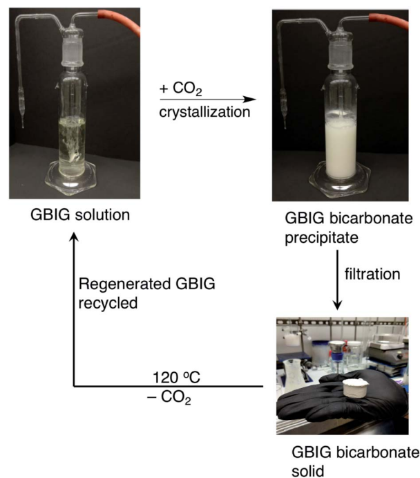
Fig. 7 \text{CO}_2 separation via GBIG bicarbonate crystallization. A flue gas simulant (12.8% \text{CO}_2 , EPA standard) is bubbled through an aqueous GBIG solution, leading to crystallization of GBIG bicarbonate. The solid is collected by filtration, then heated at 120^\circ\text{C} to release the \text{CO}_2 and regenerate the GBIG sorbent. The filtrate containing the residual GBIG, and the regenerated GBIG solid are recycled.
