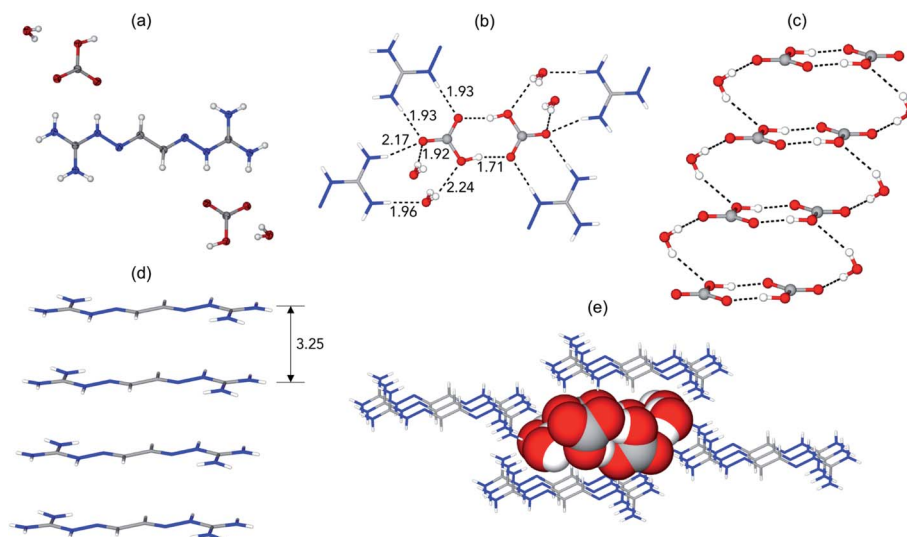
Fig. 6 X-ray crystal structure of GBIG–HCO 3 . (a) ORTEP representation, with 50% ellipsoids. (b) Hydrogen bonding of bicarbonate dimers, with contact distances shown in Å. (c) Ladder-shaped hydrogen-bonded [(HCO 3 − ) 2 (H 2 O) 2 ] n anionic cluster. (d) Stack of GBIGH 2 2+ cations, with the mean distance between adjacent cations shown in Å. (e) Crystal packing viewed along the crystallographic a axis, with the cationic stacks (shown as stick models) flanking the anionic cluster (shown as space-filling model). Reproduced with permission from ref. 41. Copyright (2019) Elsevier.
