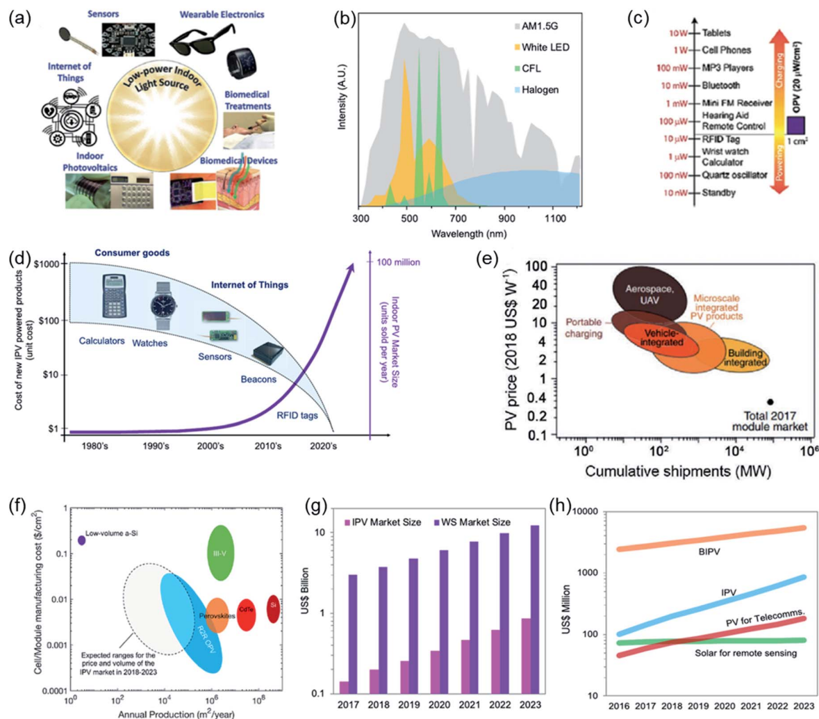
Fig. 1 (a) The equipment obtains energy through IPV's power generation under indoor lighting conditions. Reproduced from ref. 39 with permission from the [Wiley-VCH], copyright [2018]. (b) Emission spectra of different light sources. Reproduced from ref. 45 with permission from the [Elsevier], copyright [2019]. (c) Powered by IPV's of 1 square centimeter under indoor lighting and the corresponding drivable electronic equipment. Reproduced from ref. 39 with permission from the [Wiley-VCH], copyright [2018]. (d) The cost and market size of IPV's as a function of time (years). (e) Expected market size of different photovoltaic applications (2018–2027). (f) Manufacturing cost and annual production scale and indoor usage of different types of IPV's. (g) forecast of IPV's and WS market size, and (h) market demand for photovoltaic cells/modules in different energy demand fields (2016–2023). Reproduced from ref. 45 with permission from the [Elsevier], copyright [2019].
