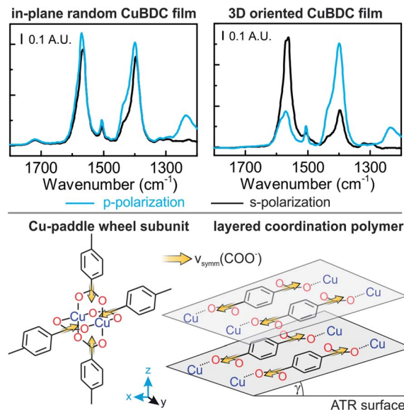
Fig. 8 (Top) Polarization-dependent ATR spectra of CuBDC prepared from random and aligned Cu(OH) 2 . Background spectrum = blank Si ATR crystal. (Bottom) Cu-paddle wheel subunit found in 2D MOFs and BDC linker alignment in a layered coordination polymer. The transition dipole moment of the ν sym (COO - ) bands are indicated by yellow arrows.
