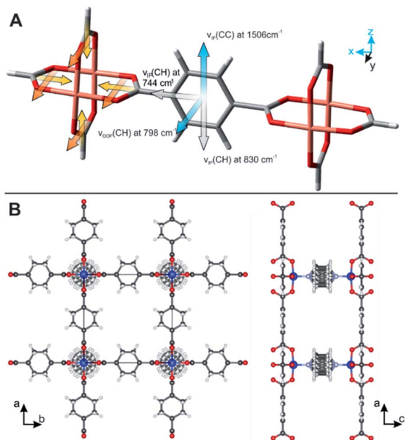
Fig. 7 (A) Illustration of the transition dipole moments for the aromatic vibrations found in the BDC linker. (B) Crystal structure of Cu 2 -(BDC) 2 DABCO with the proposed aromatic linker orientation perpendicular to the carboxylate plane.
