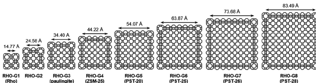
Fig. 6 Framework representations of cross sections (ca. 12 Å thick) of RHO-G1 to RHO-G8 in the RHO family of embedded isorectical zeolites. 66 Reproduced from ref. 66 with permission from the John Wiley & Sons, Inc., copyright 2016.
