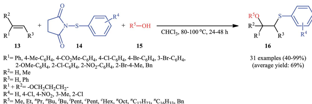
Scheme 5 Catalyst-free oxysulfenylation of alkenes 13 with 1-(aryltio)pyrrolidine-2,5-diones 14 and alcohols 15 .
