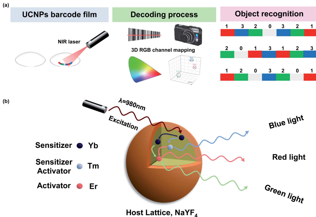
Fig. 1 (a) Schematic illustration for a NIR encoding transparent UCNP barcode film embedded in a contact lens as a model system for wearable individual recognition, the decoding process with a CCD camera through RGB value analysis, and the relevant object recognition according to the assigned codes under 980 nm NIR light. (b) Schematic illustration for the upconversion mechanism of RGB visible light emitting UCNP.
