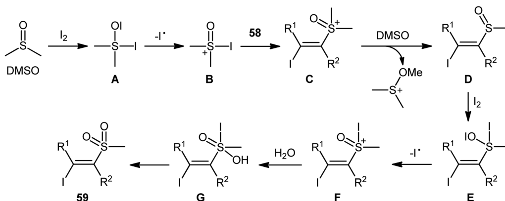
Scheme 27 Possible pathway of ( E )-α-iodo-β-methylsulfonylalkenes 59 formation.
