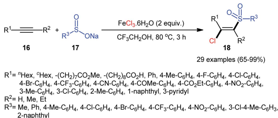
Scheme 8 Synthesis of ( E )-β-chlorovinyl sulfones 18 via three-component reaction between alkynes 16 , sodium sulfinates 17 and \text{FeCl}_3 \cdot 6\text{H}_2\text{O} .
