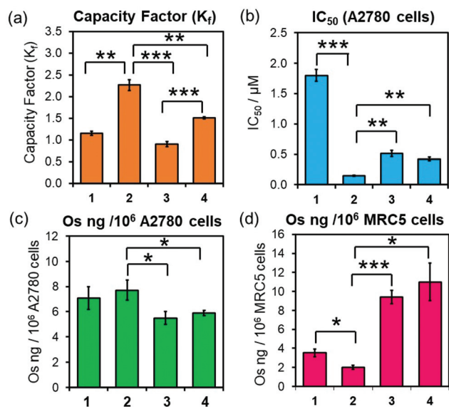
Fig. 2 (a) HPLC capacity factors ( K_f , orange) of 1–4 relative to uracil (1 : 1 v/v water:acetonitrile, 50 mM NaCl). (b) IC_{50} /μM (blue) of 1–4 in A2780 (human ovarian) cancer cells upon 24 h exposure, followed by 72 h recovery in complex-free media. (c) Cellular accumulation of ^{189}Os (ng per 10^6 per cells, green) in A2780 cells treated with 1 \times IC_{50} of 1–4 for 24 h (no recovery). (d) Cellular accumulation of ^{189}Os (ng per 10^6 per cells, pink) in MRC5 (healthy lung) fibroblasts treated with 1 \times A2780 IC_{50} of 1–4 for 24 h (no recovery). Error bars show the standard deviation from the mean. Statistical analysis was performed using Welch's unpaired t-test (assuming unequal variances): * p < 0.05 ; ** p < 0.01 ; *** p < 0.001 .
