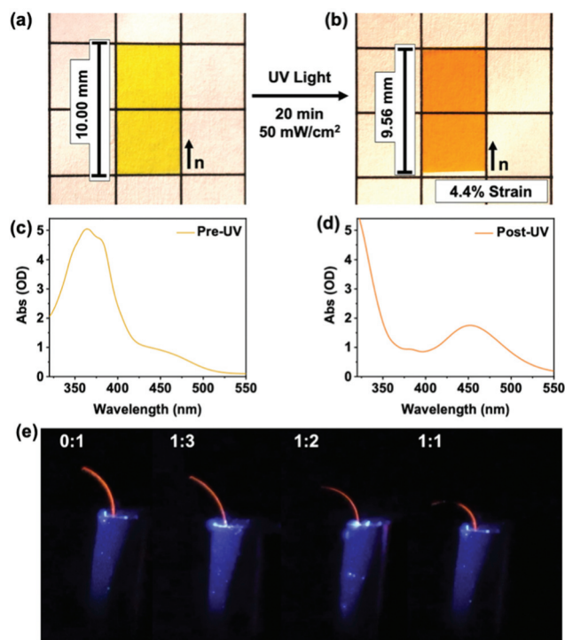
Fig. 6 Images of azobenzene-functionalized LCE (1 : 2 composition) (a) before and (b) after UV light exposure (365 nm, 20 min, 50 mW cm -2 ). UV-Vis spectra for film (c) before and (d) after UV exposure. (e) Monodomain azobenzene-functionalized LCE cantilevers (0.005 mm × 1 mm × 6 mm, increasing C6BAPE concentration from left to right) after 2 seconds of 365 nm light exposure (50 mW cm -2 ).
