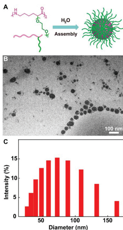
Fig. 8 Self-assembly of amphiphilic poly(OEGCL) into micelles. (A) Illustration on the formation of micelles. (B) TEM image of the micelle sample drop deposited from H_2O onto a carbon-coated copper grid; scale bar = 100 nm. (C) Size distribution of micelles measured by DLS. Reproduced from ref. 27 with permission from the American Chemical Society, copyright 2018.
