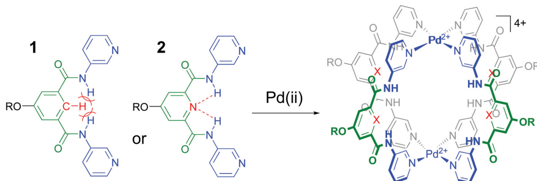
Fig. 1 Ligands 1 and 2 used in this study to make [\text{Pd}_2(\text{Ligand})_4]^{4+} complexes. R = solubility group = -(\text{CH}_2)_2\text{O}-p\text{-Ph}-C(p\text{-tBu-Ph})_3 . See section S2† for synthetic details and see Fig. S52† for a model of the steric clash present in 1 .
