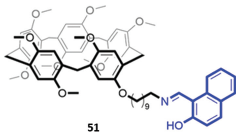
Fig. 27 Structure of pillar[5]arene receptor 51 functionalised with a 2-(hydroxy)-naphthyl imino fluorophore (in blue).
