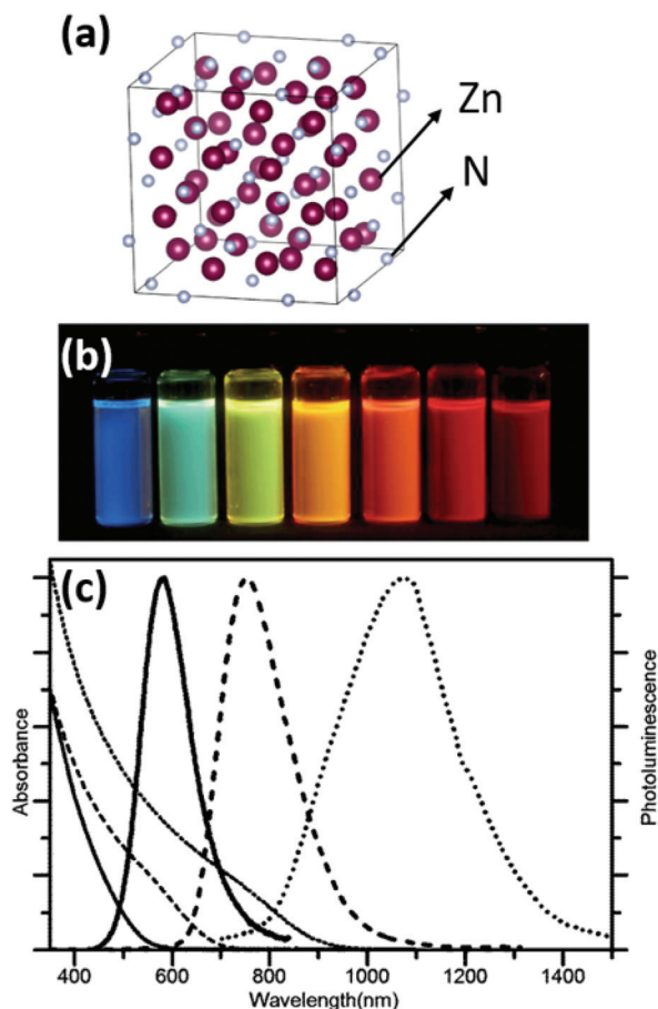
Fig. 19 (a) Crystal structure of Zn_3N_2 metal nitride. The metal is represented in purple and the nitrogen atom in grey. Structures plotted using VESTA. 48 Cif file obtained from ref. 130. (b) Toluene solutions of OLAm capped Zn_3N_2 NCs sampled at different reaction times and excited with a 365 nm lamp. (c) Absorption (thin lines) and emission (thick lines) spectra of Zn_3N_2 NCs with mean diameters of 2.1 \pm 0.4 nm (solid lines), 4.6 \pm 2.3 nm (dashed lines) and 7.1 \pm 2.0 nm (dotted lines). Reproduced from ref. 136 with permission from the Royal Society of Chemistry.
