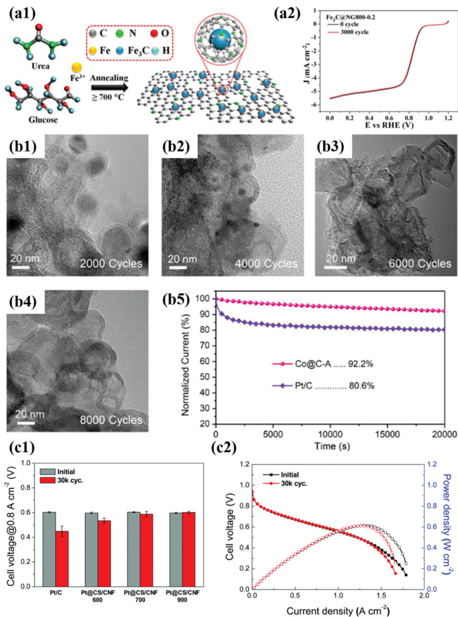
Fig. 10 (a1) Schematic illustration of synthesis of \text{Fe}_3\text{C}@\text{NG} (a2) ORR curves of the \text{Fe}_3\text{C}@\text{NG}800 before and after 3000 cycles in \text{O}_2 -saturated 0.1 M KOH solution, reproduced with permission from ref. 164, ACS copyright 2015. (b1–4) TEM images of Co@C-A before and after ADT. (b5) Chronoamperometry of Co@C-A for 20 000 s compared to commercial Pt/C in \text{O}_2 -saturated 0.1 M KOH, reproduced with permission from ref. 97, Wiley copyright 2019. (c1) Cell voltages measured at 0.1 \text{ A cm}^{-2} of MEAs before and after ADT. (c2) Polarization curves of Pt@CS/CNF900 before and after ADT, reproduced with permission from ref. 162, RSC copyright 2019.
