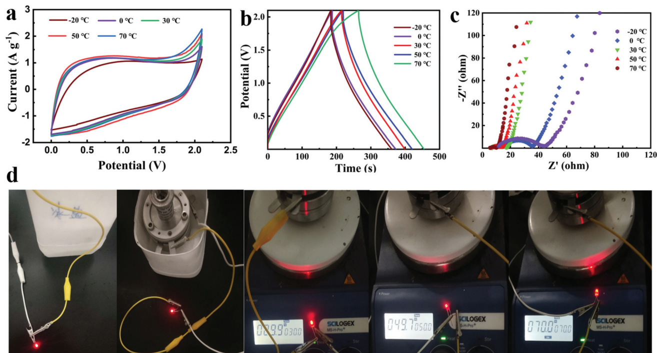
Fig. 5 The NG//NG quasi-solid-state supercapacitor with the PAAK/CMC-24 M polyelectrolyte hydrogel working at different temperatures: CV curves at 10 mV s^{-1} (a), GCD curves at 0.5 A g^{-1} (b), EIS (c), LED powered (d).
