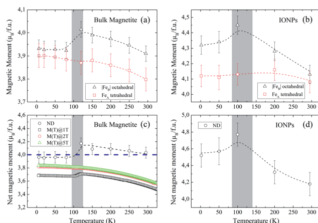
Fig. 5 Thermal variation of the \text{Fe}_{A,B} magnetic moment for (a) bulk magnetite and (b) IONP samples. Thermal evolution of the net magnetic moment per formula unit (f.u.) for (c) bulk magnetite and (d) IONPs. The blue dashed line corresponds to the theoretical net moment value for stoichiometric magnetite. Dashed lines are guides to the eye.
