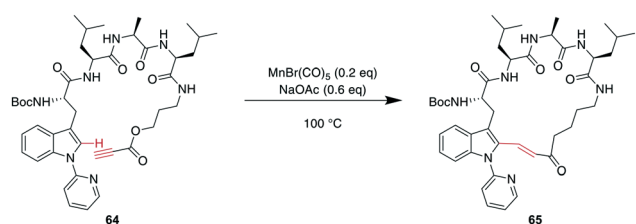
Scheme 24 Propargylic esters can be hydroarylated with N -(2-pyridyl)-derivatised Trp under Mnl catalysis to yield macrocyclic 3-indolyl acrylates.
