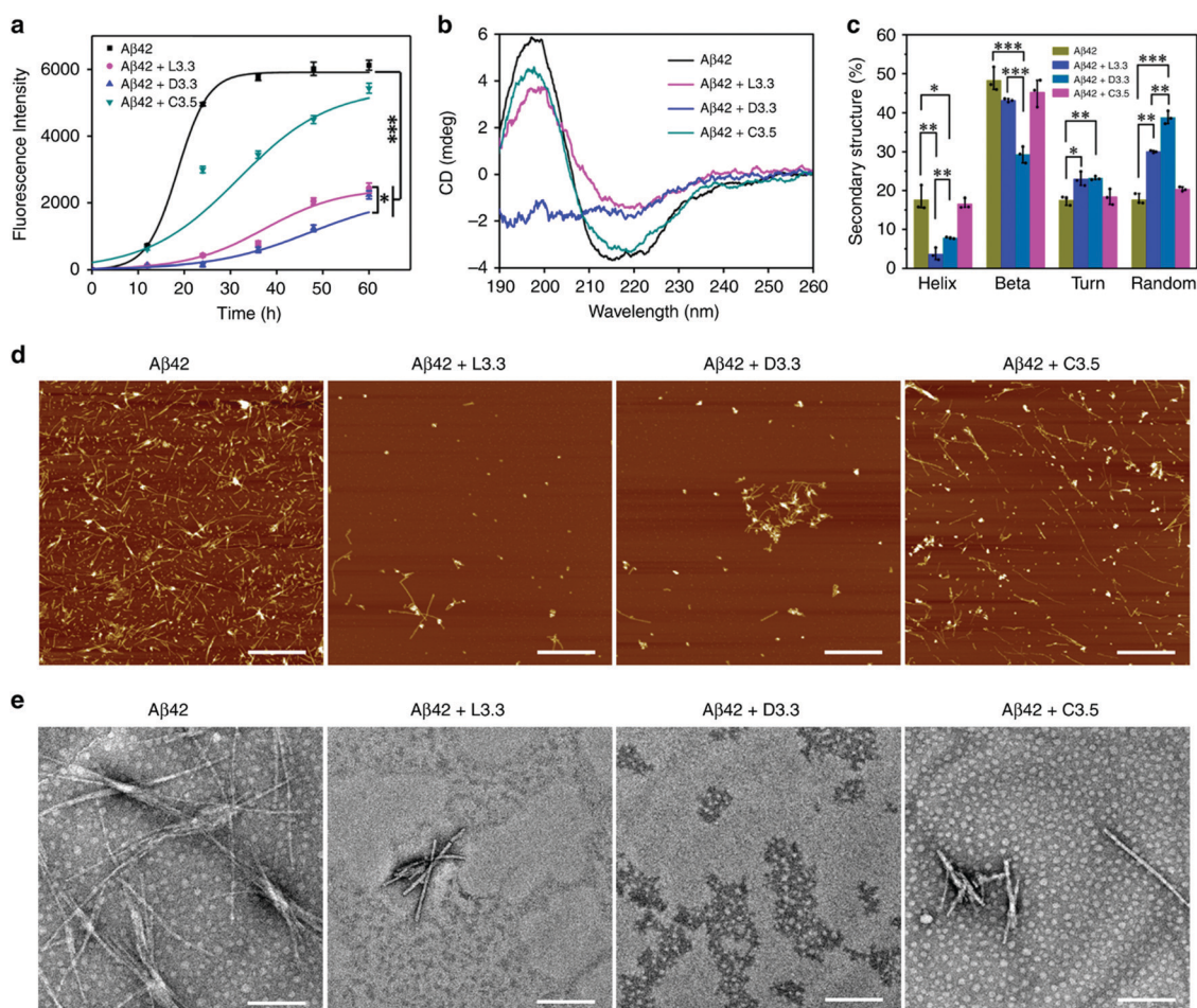
Fig. 18 (a) Fluorescence spectra of A\beta 2 illustrate a considerable reduction of up to 63% in the maximum ThT intensity for ( A\beta 42 + D3.3) and 60% for ( A\beta 42 + L3.3). (b) CD spectra of A\beta 2 show a positive peak at 195 nm and a negative peak at 215 nm, indicating the formation of the \beta -sheet structure, and a considerable reduction in both peaks was obtained on the addition of chiral Au NPs. (c) The intactness of protein secondary structure, (d) AFM images of free A\beta 2 and with L3.3, D3.3, and (e) TEM images of free A\beta 2 and with L3.3, D3.3. Reprinted with permission. 127 Copyright 2020, Springer Nature.
