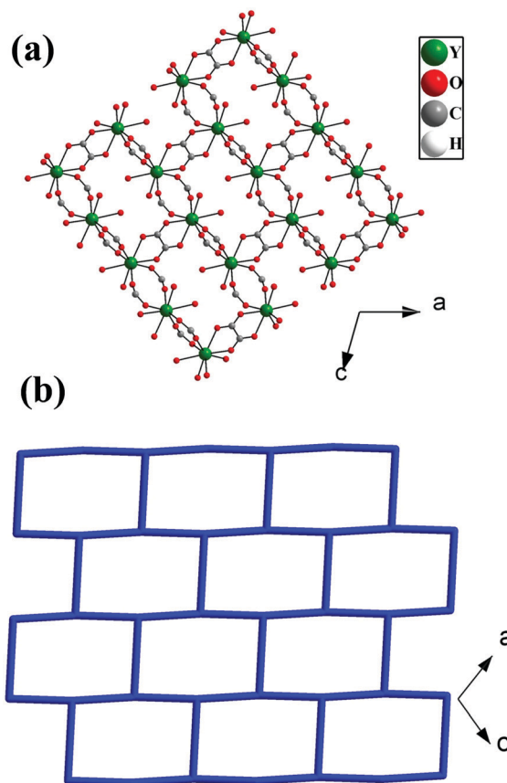
Fig. 1 (a) The 2D structure of [\text{Y}(\text{tp})(\text{ox})_{0.5}(\text{H}_2\text{O})_2] \cdot \text{H}_2\text{O} , 1 , formed by the connectivity of \text{Y}^{3+} ions and carboxylates of terephthalates and oxalates, (b) the 2D brick-wall topology based on three-connected \text{Y}^{3+} nodes.
