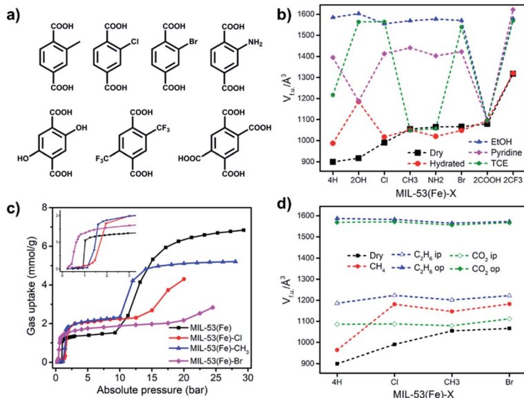
Fig. 8 (a) The functionalised bdc ligands used to synthesise MIL-53(Fe)-X variants; (b) and (d) volume per formula unit ( V_{f.u.} ) of MIL-53(Fe)-X variants under different conditions, 4H = \text{MIL-53(Fe)} ; (c) \text{C}_2\text{H}_6 sorption isotherms of MIL-53(Fe)-X at 303 K.
