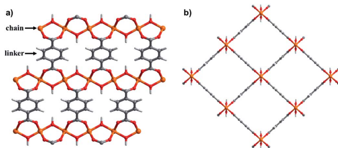
Fig. 5 Crystal structures of MIL-53(M): (a) MO_4(OH)_2 chains connected by bdc linkers; (b) 1D rhombic channels in the open phase, guest molecules are omitted for clarity. Orange: M (Cr, Al, Fe, etc.), red: O, grey: C, light grey: H.
