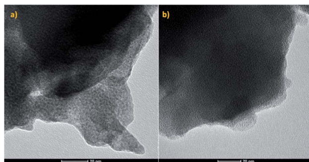
Fig. 1 TEM micrographs of (a) pristine UiO-66(Zr) and (b) \text{NH}_2\text{-UiO-66(Zr)} loaded with Cu nanoclusters.
