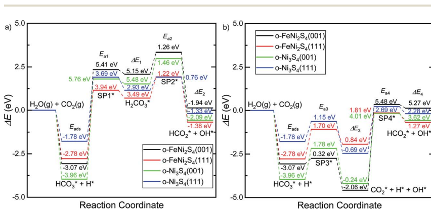
Fig. 5 Minimum energy pathways for \text{CO}_2 reduction by \text{H}_2\text{O} via (a) substitution and (b) dissociation mechanisms on the (001) and (111) surfaces of the o\text{-FeNi}_2\text{S}_4 and o\text{-Ni}_3\text{S}_4 thiospinels. Minimum states and saddle points are denoted by horizontal lines linked by dashed lines. Energies are referenced to the isolated \text{H}_2\text{O} and \text{CO}_2 molecules as well as the surface slab. Adsorbed species are denoted using the symbol *. Adsorption energies ( E_{\text{ads}} ), elemental step energies ( \Delta E_i ) and activation energies ( E_{\text{ai}} ) are also indicated.
