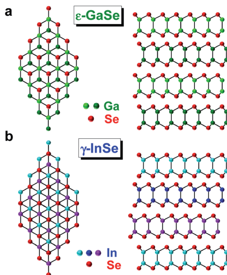
Fig. 1 Atomic structure and stacking order of (a) \epsilon -GaSe and (b) \gamma -InSe.
