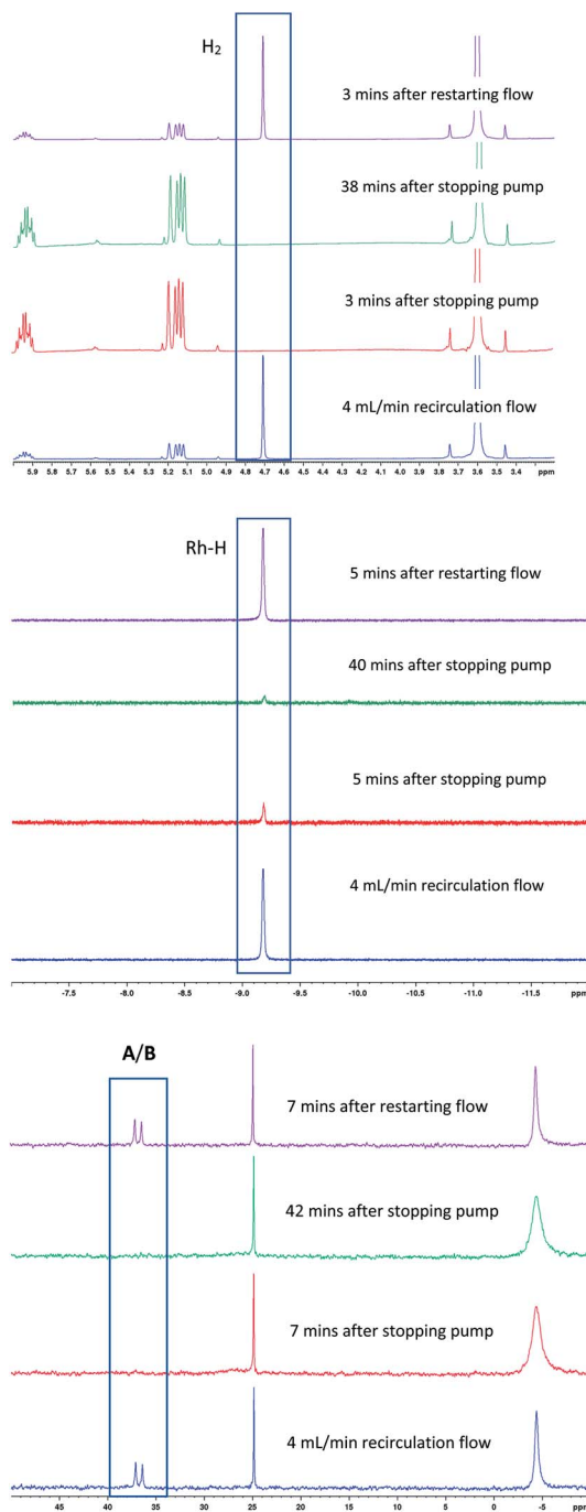
Fig. 13 ^1H and ^{31}P\{^1H\} FlowNMR spectra of [Rh(CO)_2(acac)] + 6PPh_3 catalysed hydroformylation of 1-hexene in toluene at 50 °C and 12 bar of H_2/CO (1 : 1) during stop/start cycling of flow. [Rh(CO)_2(acac)] = 2.5 mM, [1\text{-hexene}] = 500 mM, [PPh_3] = 15 mM.
