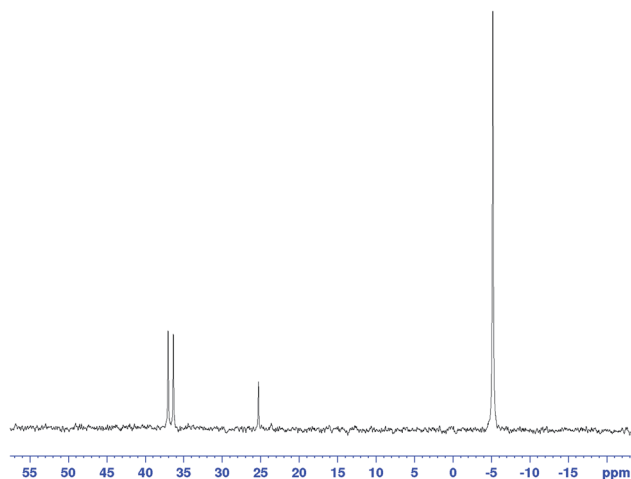
Fig. 11 ^{31}\text{P}\{\text{H}\} FlowNMR spectrum recorded during [\text{Rh}(\text{CO})_2(\text{acac})] + 6\text{PPh}_3 catalysed hydroformylation of 1-hexene in toluene at 50 °C and 12 bar of \text{H}_2/\text{CO} (1 : 1) at t = 395 min. [\text{Rh}(\text{CO})_2(\text{acac})] = 2.5 mM, [1\text{-hexene}] = 500 mM, [\text{PPh}_3] = 15 mM.
