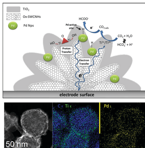
Fig. 6 Top: Graphical sketch of the PdNP/ \text{TiO}_2\text{@CNH} nano hybrid and of the interfacial synergy towards the reversible \text{HCOOH} formation; bottom: HAAFD (black and white) and EDX elemental mapping of C, Ti and Pd confirming the co-location of the three elements.
