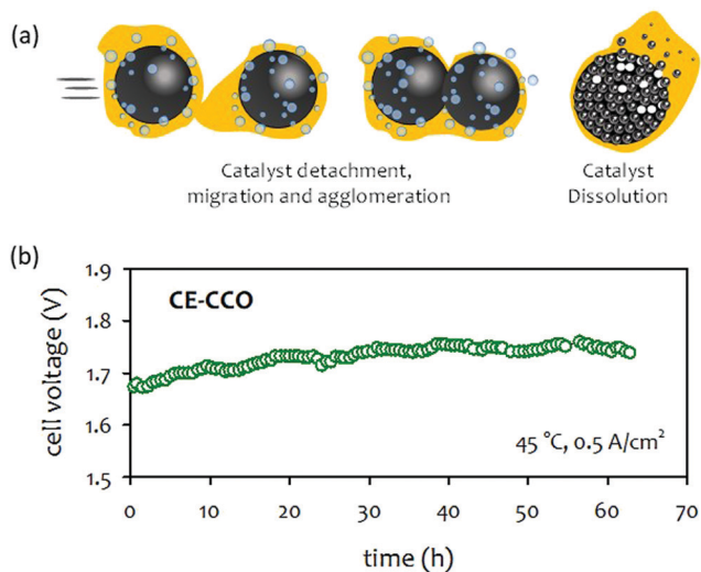
Fig. 15 (a) Catalyst degradation pathways under AEMWE operating conditions. (b) Durability of 1 M KOH-fed AEMWE at 500 \text{ mA cm}^{-2} at 45 \text{ }^{\circ}\text{C} . AEM: Sustainion ® X37-50, anode: CuCo-oxide on nickel form (CE-CCO), cathode: Pt/C ( 1 \text{ mg}_{\text{Pt}} \text{ cm}^{-2} ). 92 Adapted with permission. 92 Copyright 2020, Elsevier.
