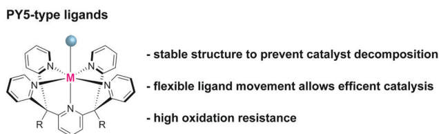
Chart 5 Summary of features of water oxidation catalysts with PY5 -type ligands.
