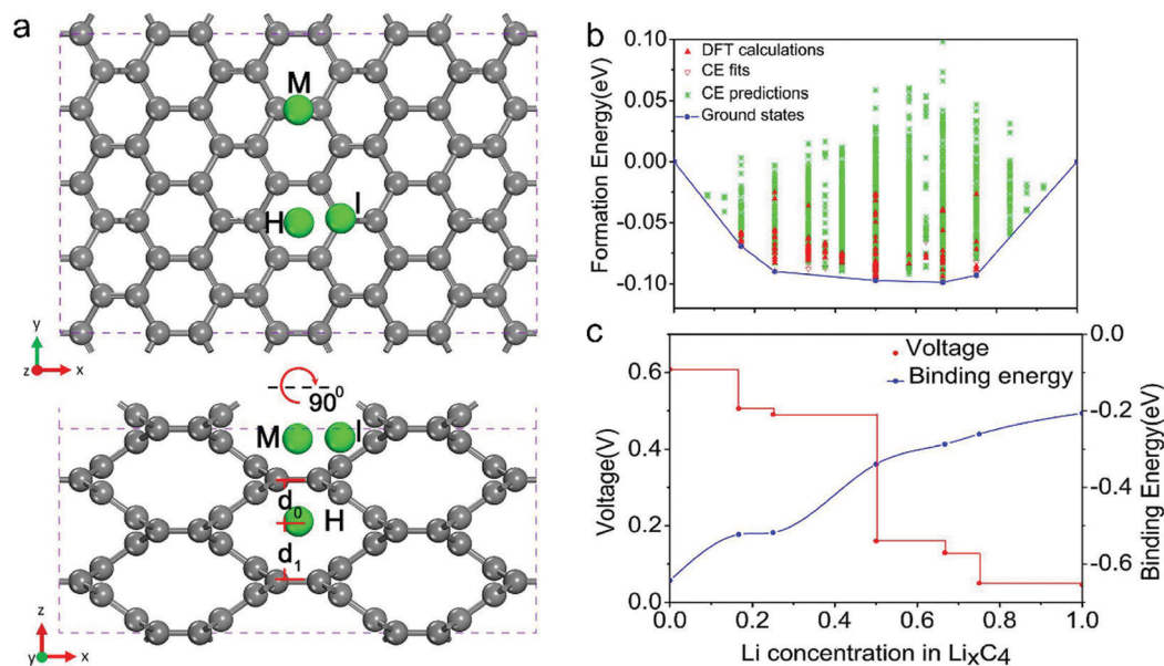
Fig. 16 (a) Structure of bco-C16 and the schematics of the possible Li-ion absorption sites in top and side view. (b) Formation energies predicted for the 150 different Li configurations with 5 stable intermediate phases. (c) Corresponding voltage profile (marked in red) and binding energy profile (marked in blue) calculated along the minimum energy path. Reproduced from ref. 298 with permission from United States National Academy of Sciences.
