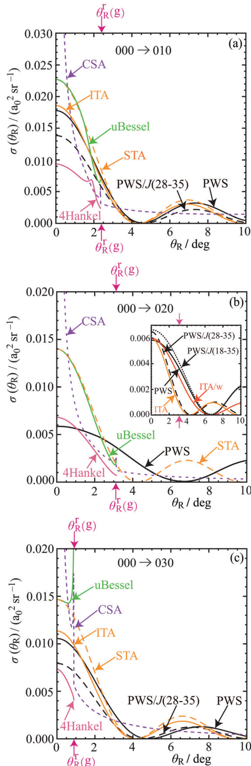
Fig. 7 Plots of \sigma(\theta_R) versus \theta_R at E_{\text{trans}} = 1.35 eV for the (a) 000 \rightarrow 010, (b) 000 \rightarrow 020, (c) 000 \rightarrow 030, transitions for the angular range, \theta_R = 0^\circ to \theta_R = 10^\circ . The DCSs plotted are: PWS (black solid curve), ITA (orange solid curve), STA (orange dashed curve), uBessel (green solid curve), 4Hankel (pink solid curve), CSA (lilac dashed curve), CSA/N (red dotted curve) and their sum, CSA (lilac dashed curve). The pink rainbow angle in the glory region is denoted, \theta_R^F(g) ; it forms the natural boundary for the uBessel, 4Hankel, and CSA/F approximations, which forms part of CSA. Also shown are DCSs, (black dashed curves) for restricted PWS for J = 28 – 35 . In the inset for (b) there are also plotted DCSs for PWS/J(18–35) (black dotted curve) and the weighted ITA, denoted ITA/w (orange solid curve).
