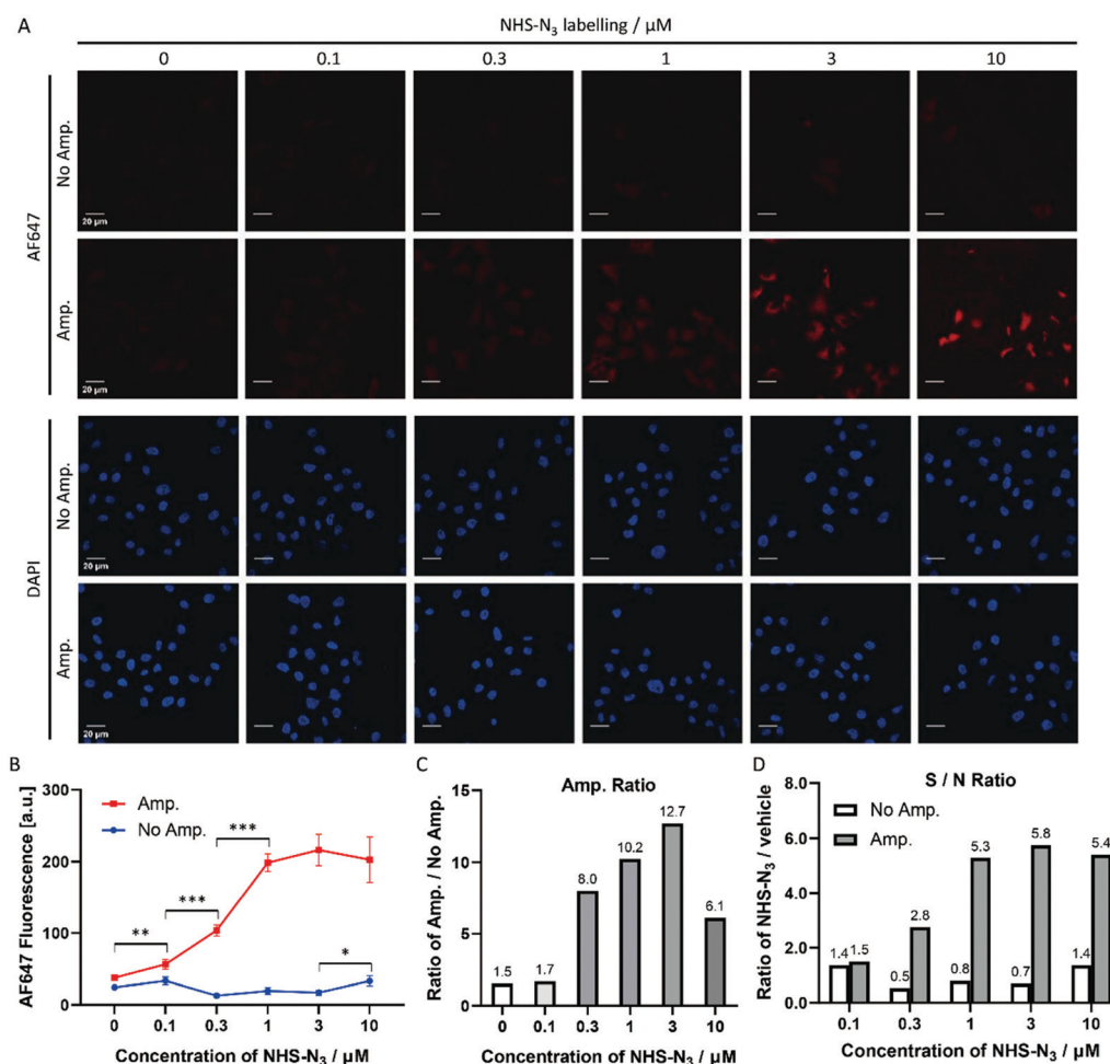
Fig. 3 Click-based amplification on fixed HeLa cells with NHS- N_3 labelling. (A) Confocal imaging of fixed HeLa cells without and with Click-based amplification (No Amp. and Amp.). HeLa cells were treated with a concentration gradient of NHS- N_3 from 0.1 \mu M to 10 \mu M. DAPI stained the nuclei of the HeLa cells. Scale bars, 20 \mu m. (B) Quantification of the cellular AF647 fluorescence intensities in (A) with ImageJ. The red line represents the fluorescence intensity of HeLa cells with Click-based amplification (Amp.), and each data point is the average fluorescence intensity of 20 cells chosen randomly from the microscopy imaging. The blue line represents the fluorescence intensity of HeLa cells without Click-based amplification (No Amp.). Error bar: the standard error (SE). (C) Amplification ratios (Amp./No Amp.). (D) Signal-to-noise ratios (NHS- N_3 /vehicle). *** p < 0.001, ** p < 0.01, * p < 0.05.
