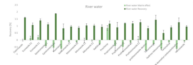
Fig. 2 SPE recovery and matrix effect of antifungal agents in river water samples (a negative value indicates ionization suppression and a positive value indicates ionization enhancement).
