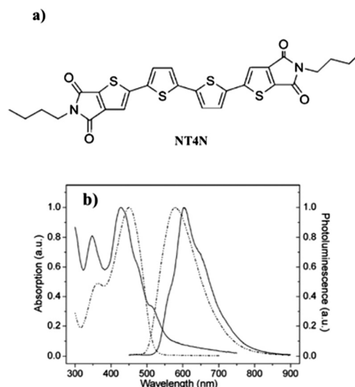
Fig. 5 (a) Molecular structure of NT4N (b) normalized absorption and emission of NT4N solution ( \text{CH}_2\text{Cl}_2 , 4 \times 10^{-5} M, dashed line) and film (100 nm thick, solid line). Adapted from ref. 63 with permission from the Royal Society of Chemistry.
