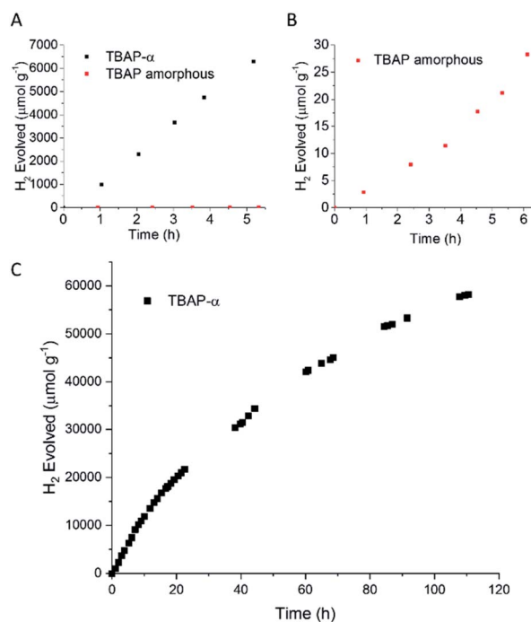
Fig. 6 (A) Time-course of hydrogen evolution for TBAP- \alpha (black symbols) and TBAP amorphous (red symbols) (25 mg) loaded with 1 wt% Pt, from photodeposition of \text{H}_2\text{PtCl}_6 , dispersed in ascorbic acid solution (25 mL, 0.1 M) illuminated with a 300 W Xe light source fitted with a \lambda > 420 nm cut-off filter. (B) Expanded plot showing activity for amorphous TBAP . (C) Extended run over 110 hours. The solution was degassed at 6, 11, 18, 40, 67 and 90 hours.
