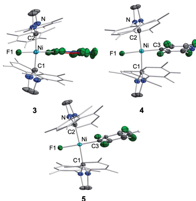
Fig. 1 Molecular structures of [\text{Ni}(\text{Mes}_2\text{Im})_2(\text{F})(\text{C}_6\text{F}_5)] (3) (top left), [\text{Ni}(\text{Mes}_2\text{Im})_2(\text{F})(2,3,5,6\text{-C}_5\text{F}_4\text{N})] (4) (top right) and [\text{Ni}(\text{Mes}_2\text{Im})_2(\text{F})(2,3,5,6\text{-C}_6\text{F}_4\text{H})] (5) (bottom) in the solid state (ellipsoids drawn at the 50% probability level). Hydrogens atoms, with exception of the proton at the fluoroaromatic of 5, are omitted for clarity.
